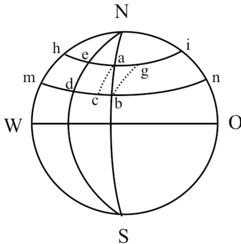
Fig. 1. Graphical reconstruction from Kant's handwritten notes of his explanation of the deflective effect of the earth's rotation.
